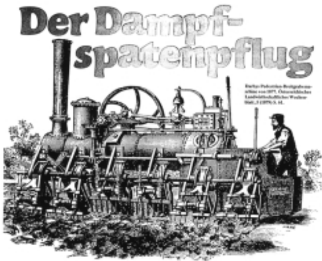
Figure 1: The Steam Spade Plough from the year 1877. Derby's Pedestrian Wide-Digging Machine from 1877 (Austrian Agrarian Weekly, 5 (1879), p. 61)
