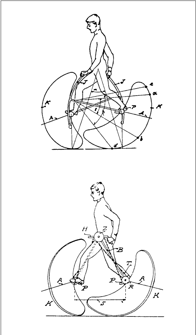
Figure 4: Curved shoes from Robert Michael (1903), a device to increase the length of one's stride (DRP 152 505).
